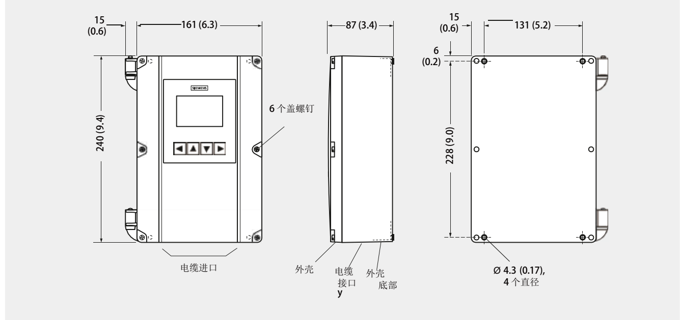
MultiRanger 200 HMI, 尺寸 mm (inch)
